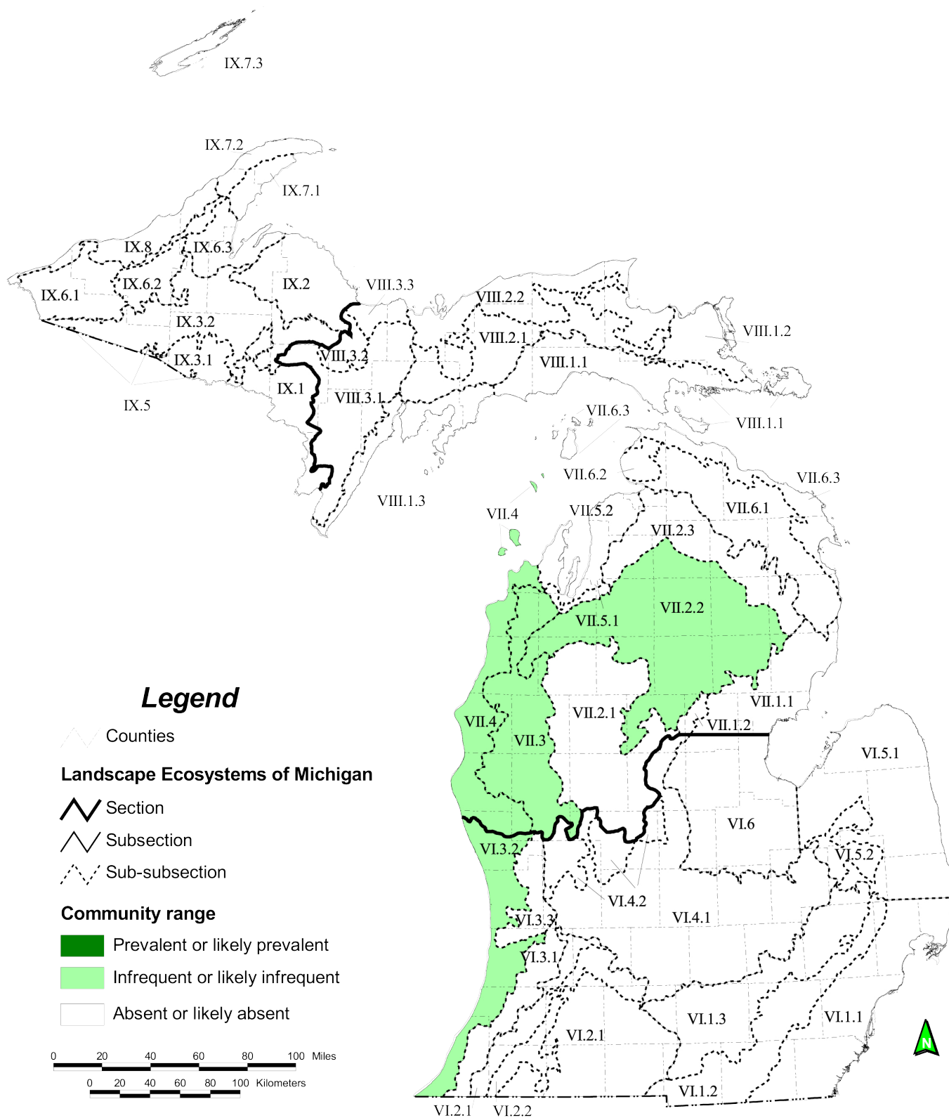
Ecoregional map of Michigan (Albert 1995) depicting distribution of wet-mesic sand prairie (Albert et al. 2008)
